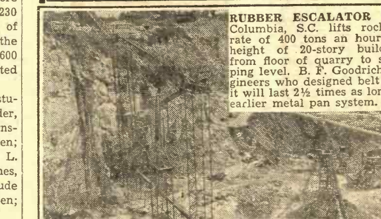
RUBBER ESCALATOR near Columbia, S.C. lifts rock at rate of 400 tons an hour the height of 20-story building, from floor of quarry to shipping level. B. F. Goodrich engineers who designed belt said it will last 2½ times as long as earlier metal pan system.
